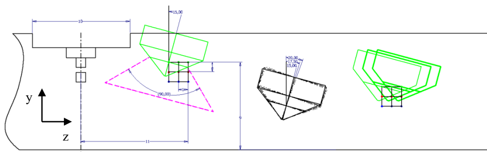
Fig. 4. The layout of the injector relative to the spark plug, together with the parameters used for the injection and combustion analysis (angle, distance)
