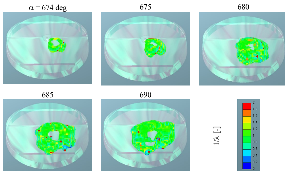
Fig. 6. Isolating the constant value of \lambda = 1 of the fuel dose development in the combustion chamber (injector position relative to the spark plug y = 7 mm, z = 10 mm, \alpha = 15^\circ )
